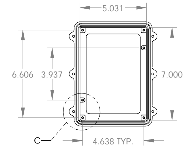
INSIDE COVER DETAILS
