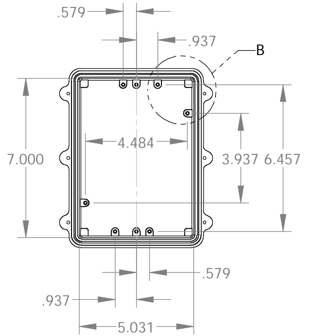
INSIDE BODY DETAILS
