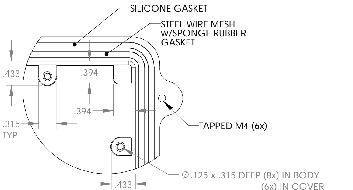
DETAIL B SCALE 4 : 1
